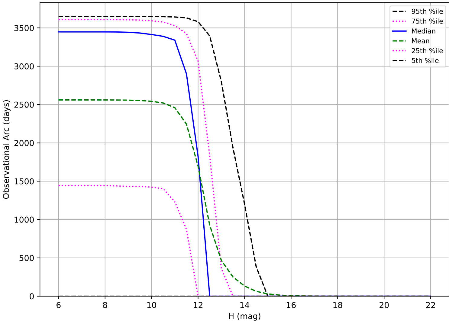
early_ss_template_fpextra3.0_v3.4_10yrs: Observational Arc Length OCC_r20
