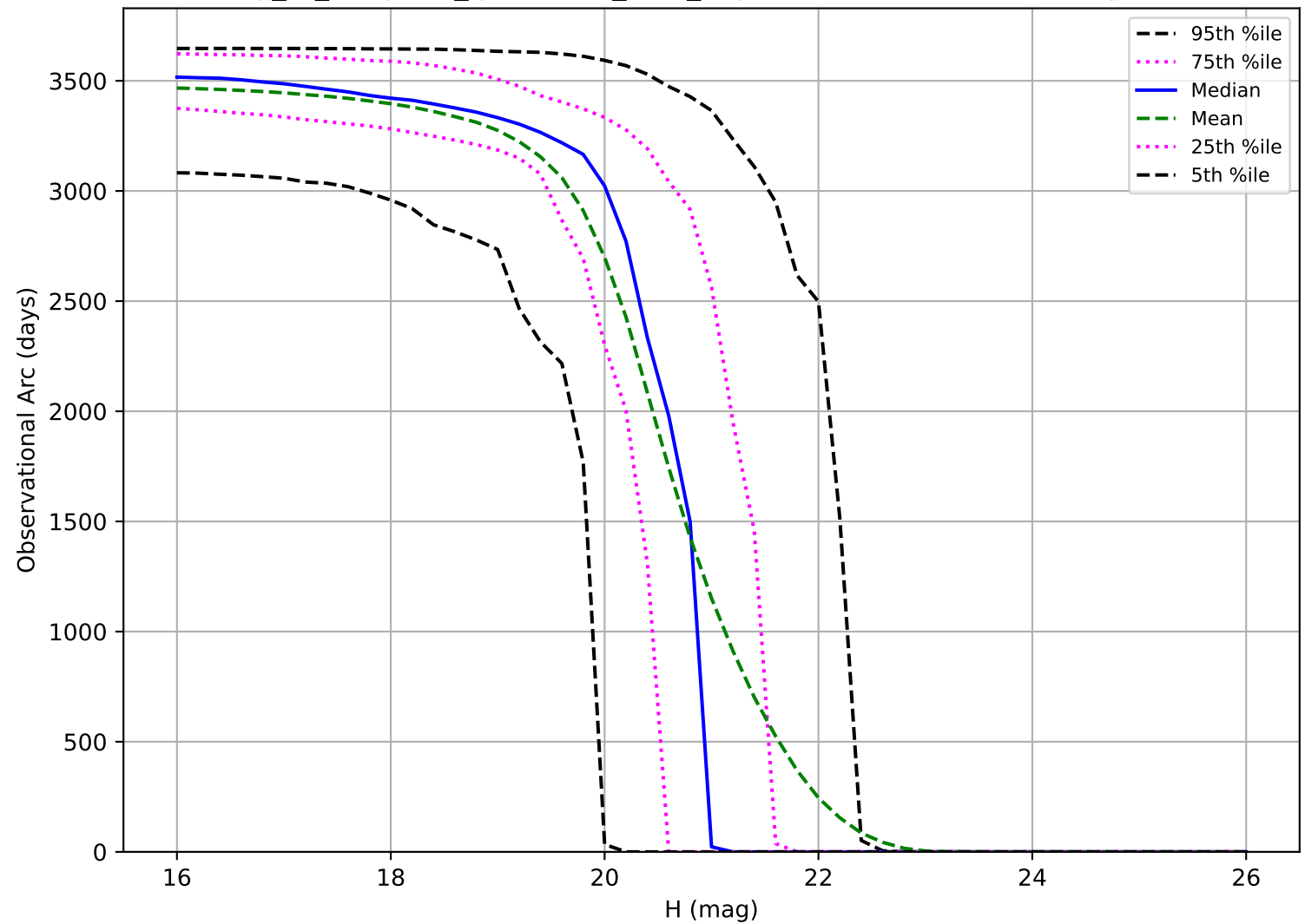
early_ss_template_fpextra3.0_v3.4_10yrs: Observational Arc Length MBA
