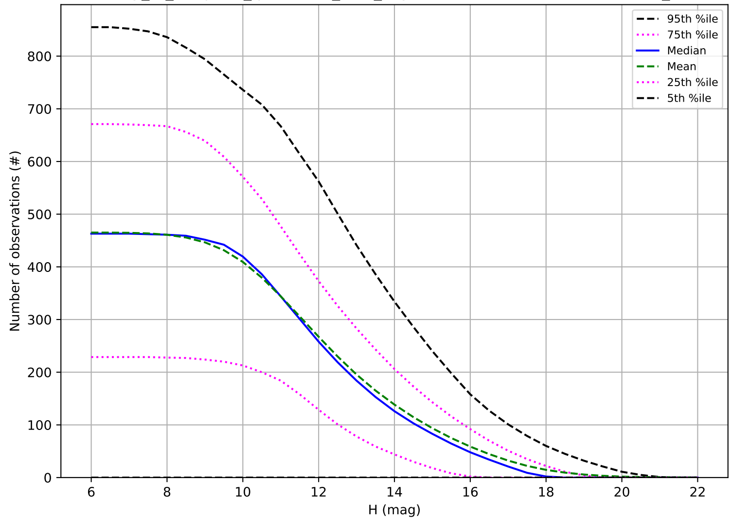
early_ss_template_fpextra3.0_v3.4_10yrs: Number of observations OCC_r5
