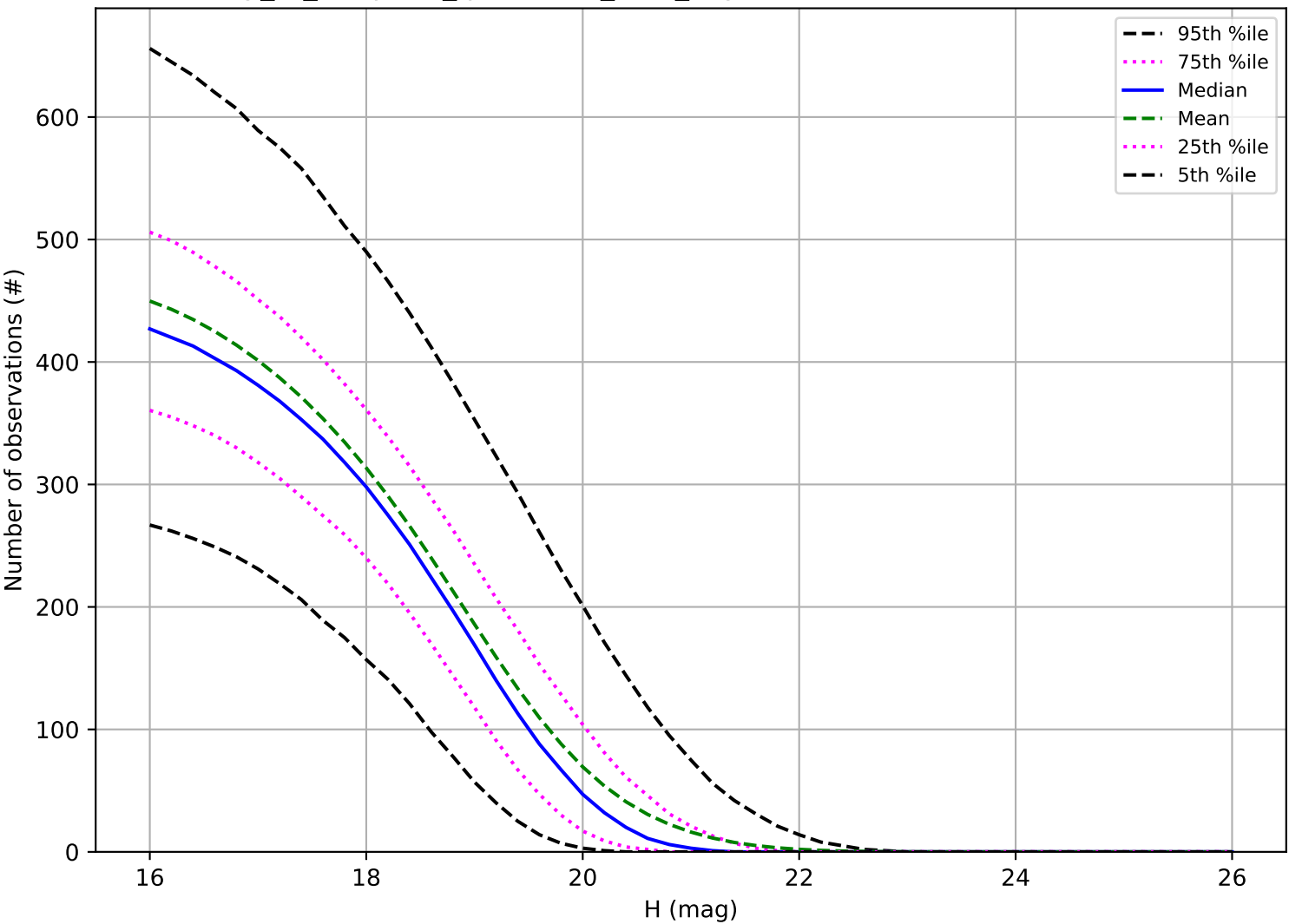
early_ss_template_fpextra3.0_v3.4_10yrs: Number of observations MBA
