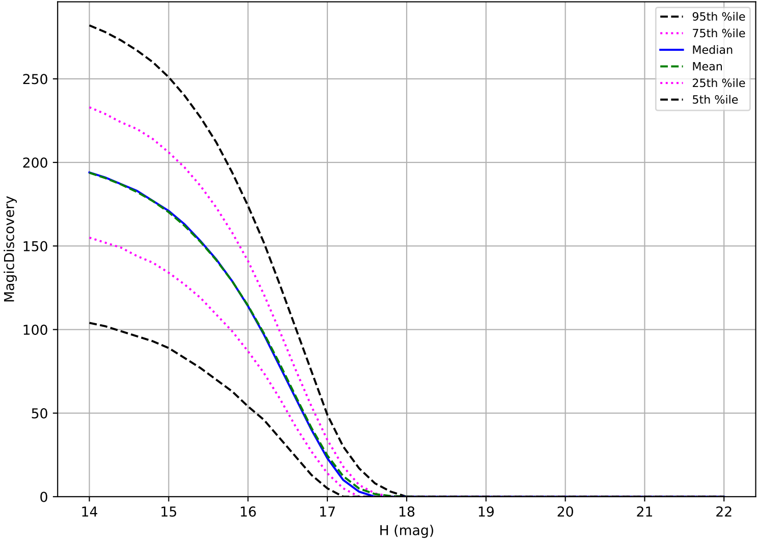
early_ss_template_fpextra3.0_v3.4_10yrs: Trojan 6 detections in 60 nights detection loss
