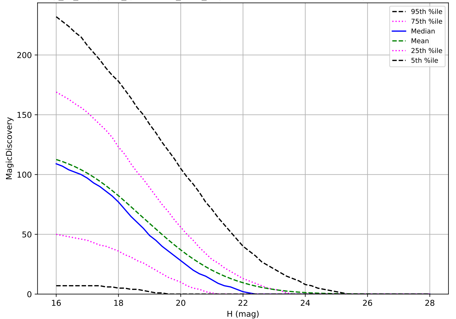
early_ss_template_fpextra3.0_v3.4_10yrs: PHA 6 detections in 60 nights detection loss
