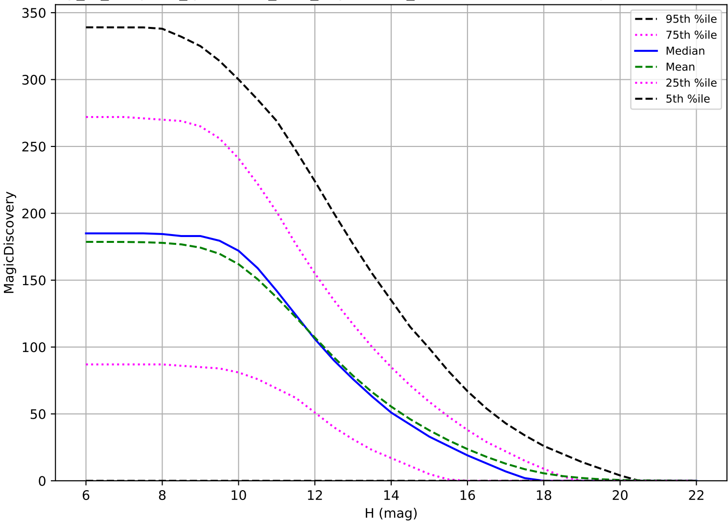
early_ss_template_fpextra3.0_v3.4_10yrs: OCC_r5 6 detections in 60 nights detection loss
