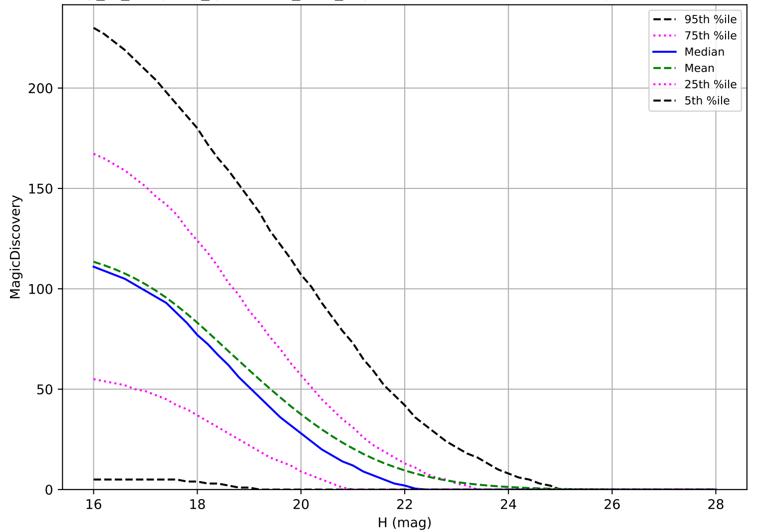
early_ss_template_fpextra3.0_v3.4_10yrs: NEO 6 detections in 60 nights detection loss
