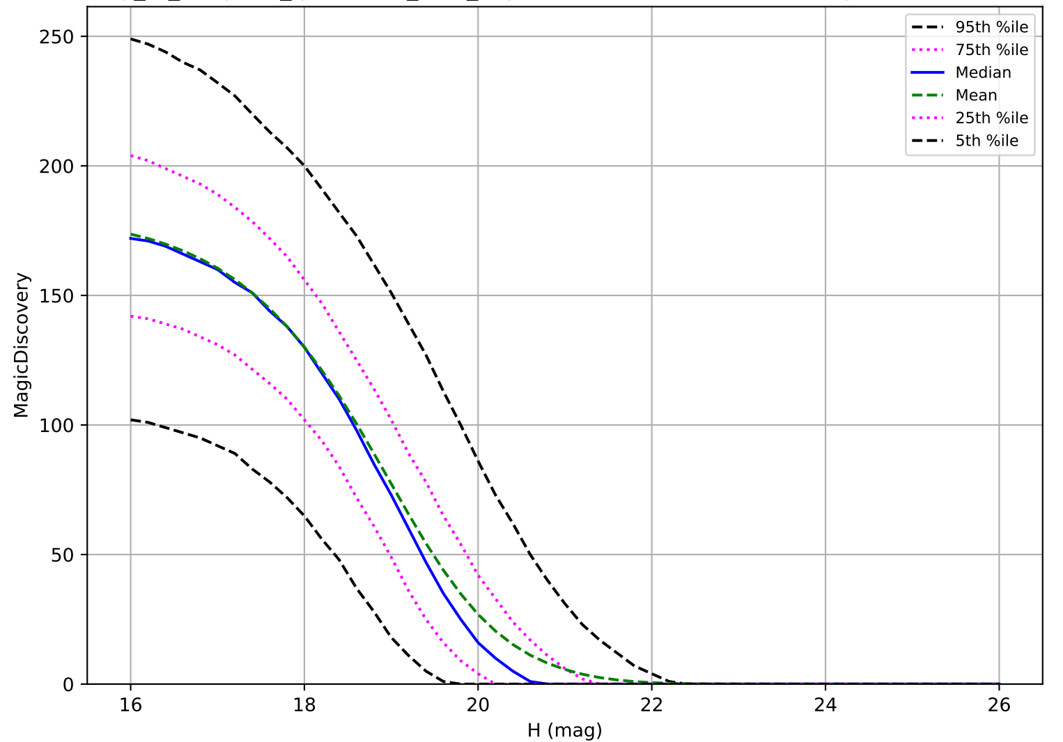
early_ss_template_fpextra3.0_v3.4_10yrs: MBA 6 detections in 60 nights detection loss
