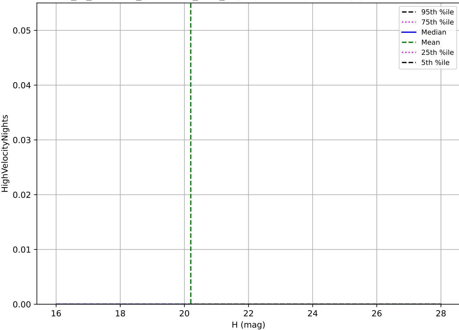
early_ss_template_fpextra3.0_v3.4_10yrs: Vatira High velocity pair detection loss
