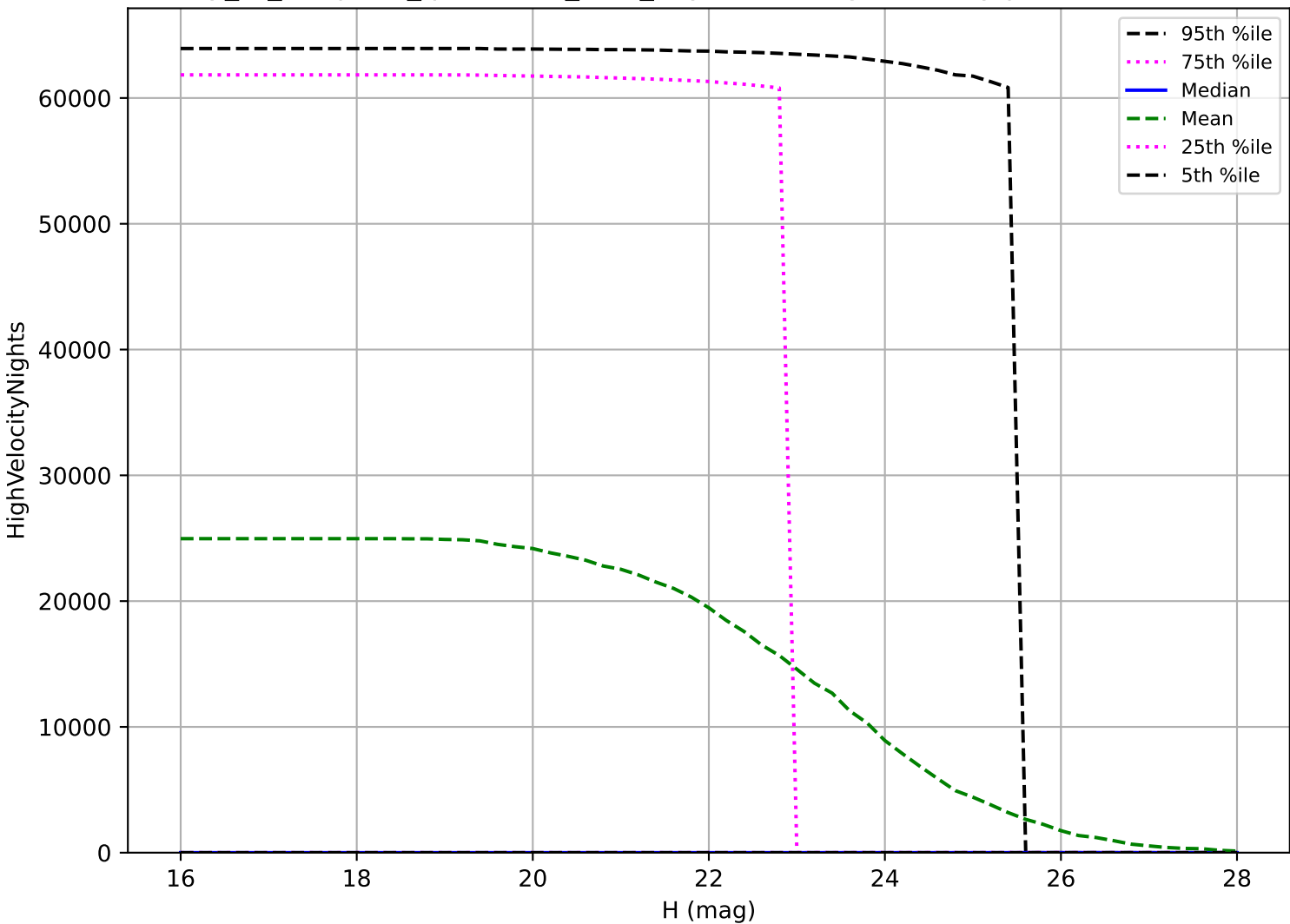
early_ss_template_fpextra3.0_v3.4_10yrs: PHA High velocity pair detection loss
