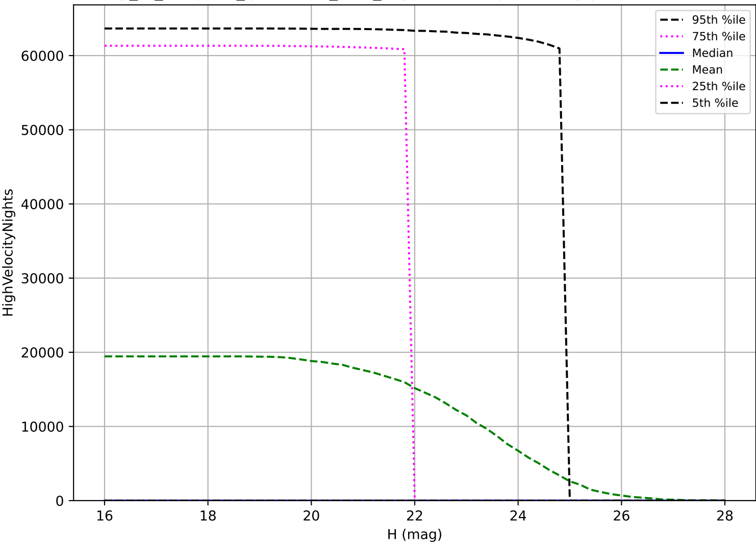
early_ss_template_fpextra3.0_v3.4_10yrs: NEO High velocity pair detection loss
