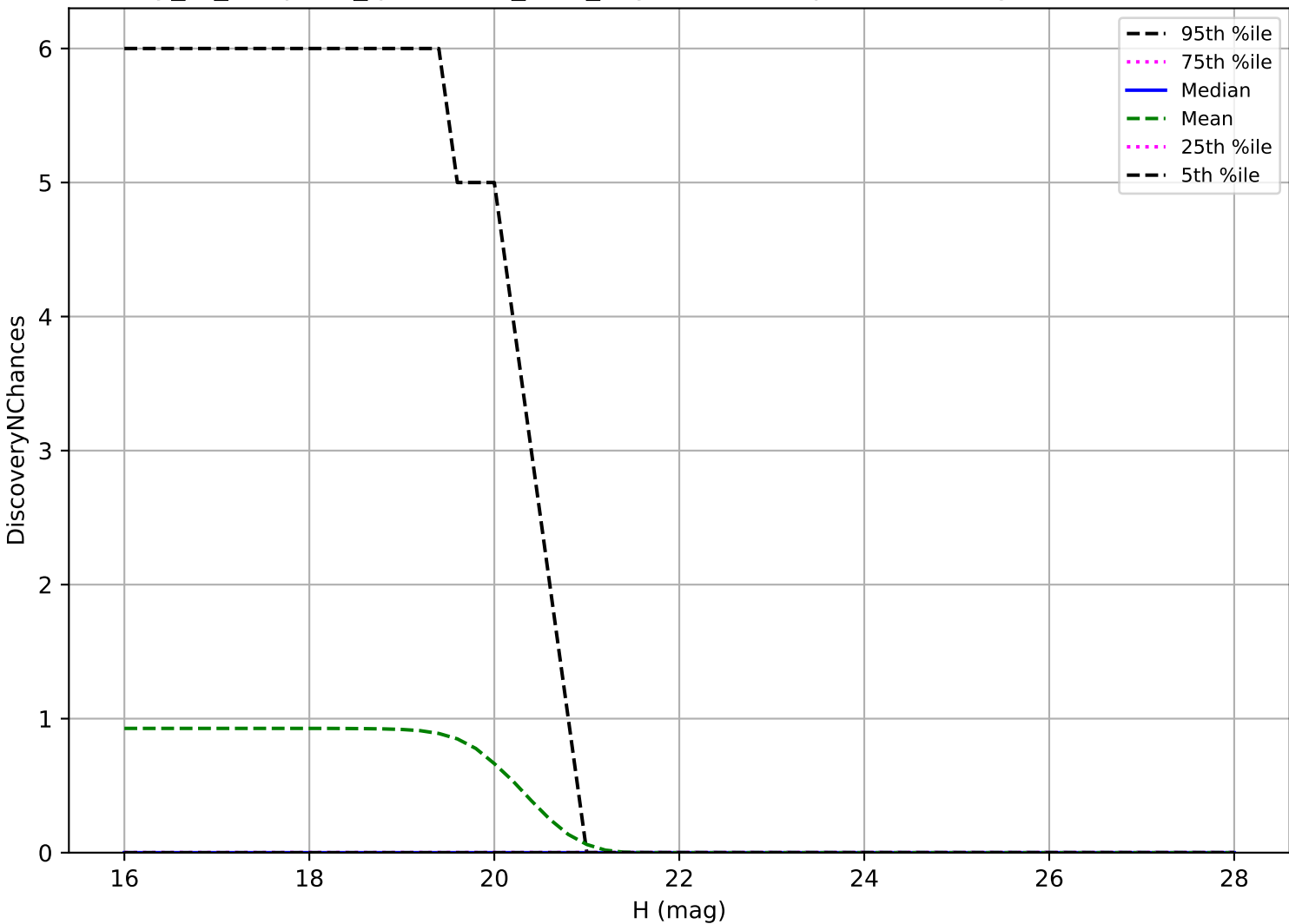
early_ss_template_fpextra3.0_v3.4_10yrs: Vatira 3 pairs in 15 nights detection loss
