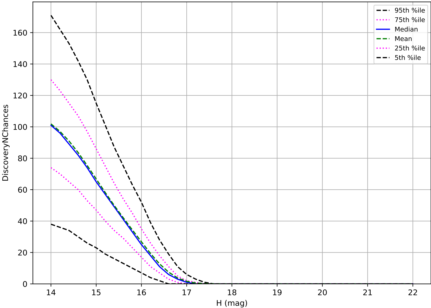
early_ss_template_fpextra3.0_v3.4_10yrs: Trojan 3 pairs in 15 nights detection loss
