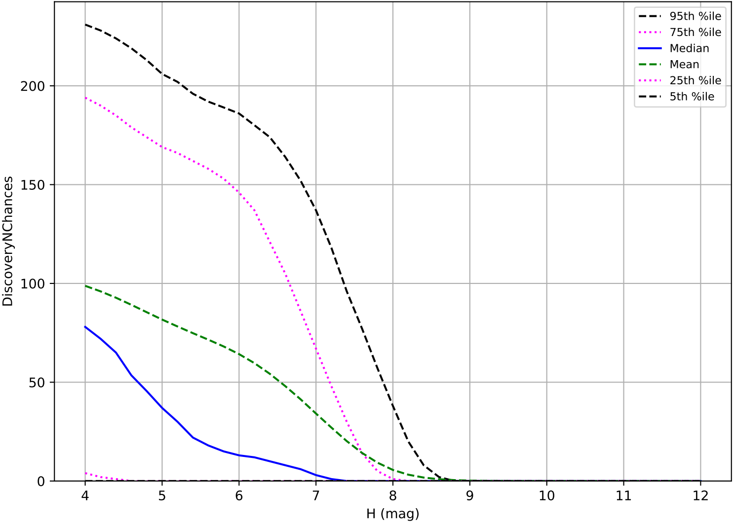
early_ss_template_fpextra3.0_v3.4_10yrs: TNO 3 pairs in 15 nights detection loss
