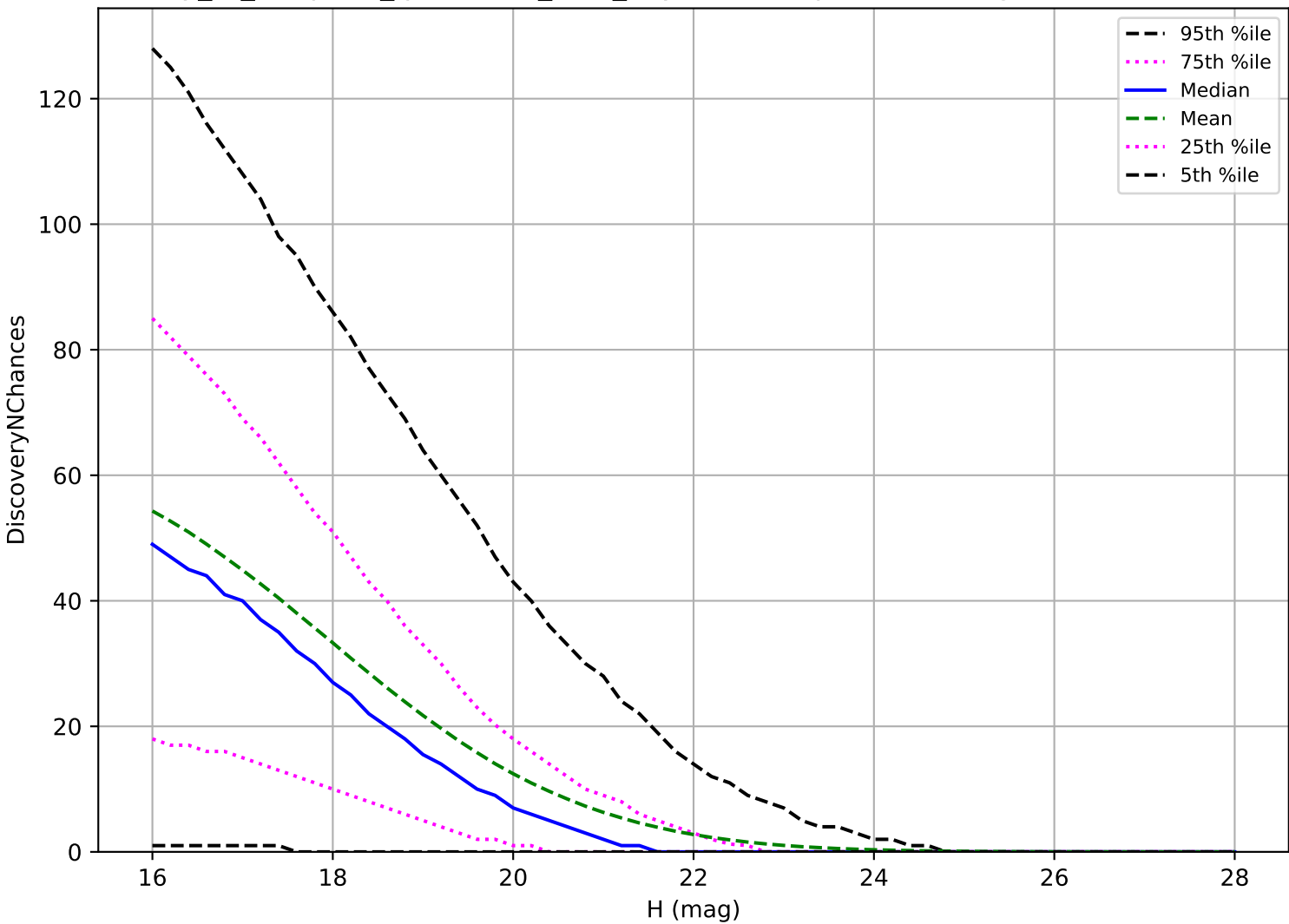
early_ss_template_fpextra3.0_v3.4_10yrs: PHA 3 pairs in 15 nights detection loss
