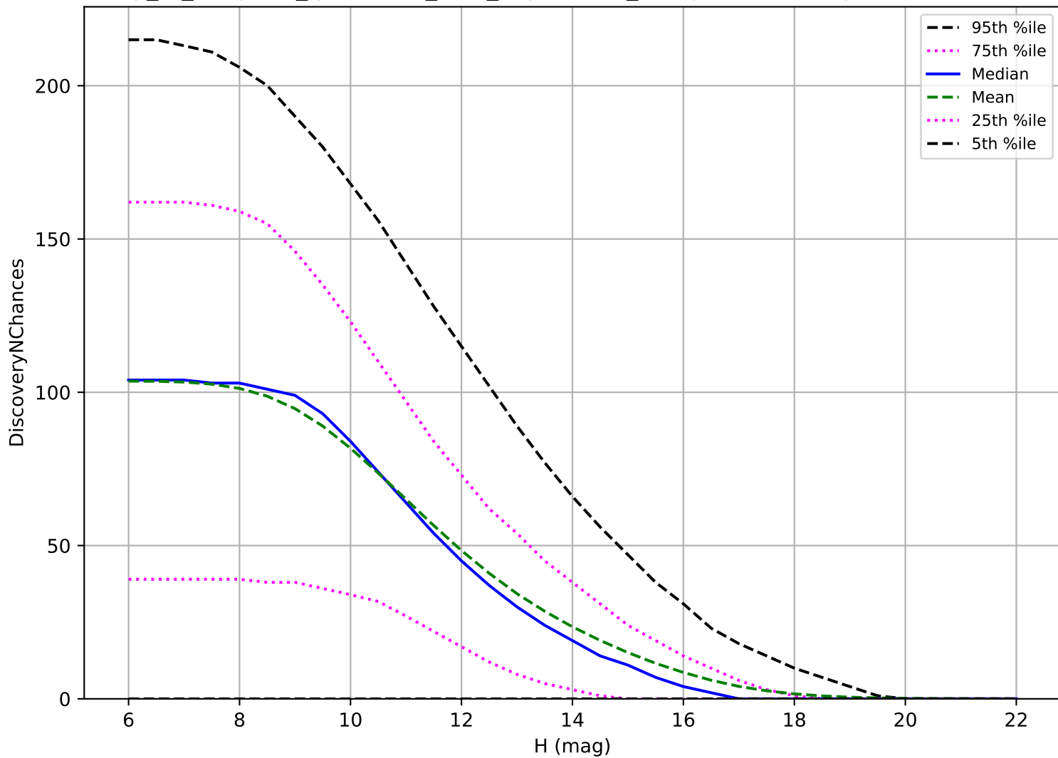
early_ss_template_fpextra3.0_v3.4_10yrs: OCC_r5 3 pairs in 15 nights detection loss
