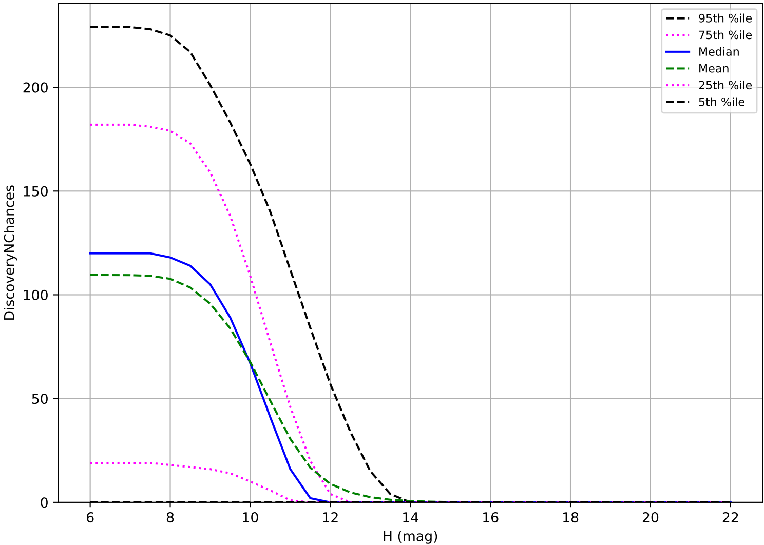
early_ss_template_fpextra3.0_v3.4_10yrs: OCC_r20 3 pairs in 15 nights detection loss
