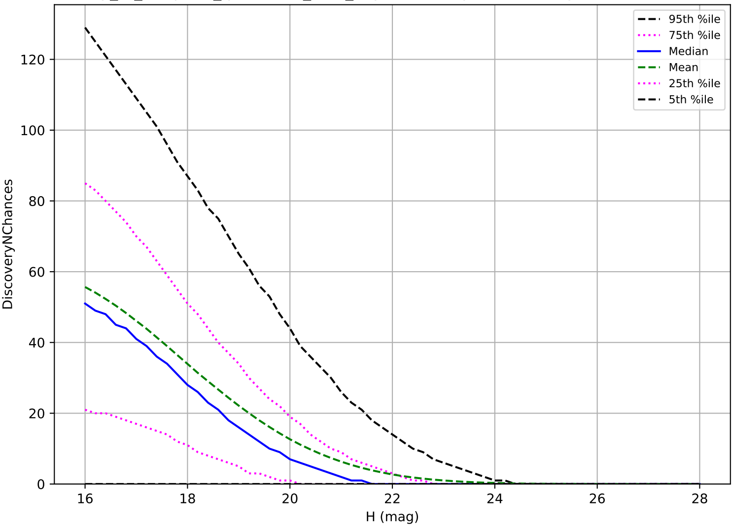
early_ss_template_fpextra3.0_v3.4_10yrs: NEO 3 pairs in 15 nights detection loss
