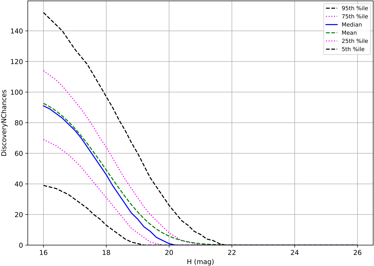
early_ss_template_fpextra3.0_v3.4_10yrs: MBA 3 pairs in 15 nights detection loss
