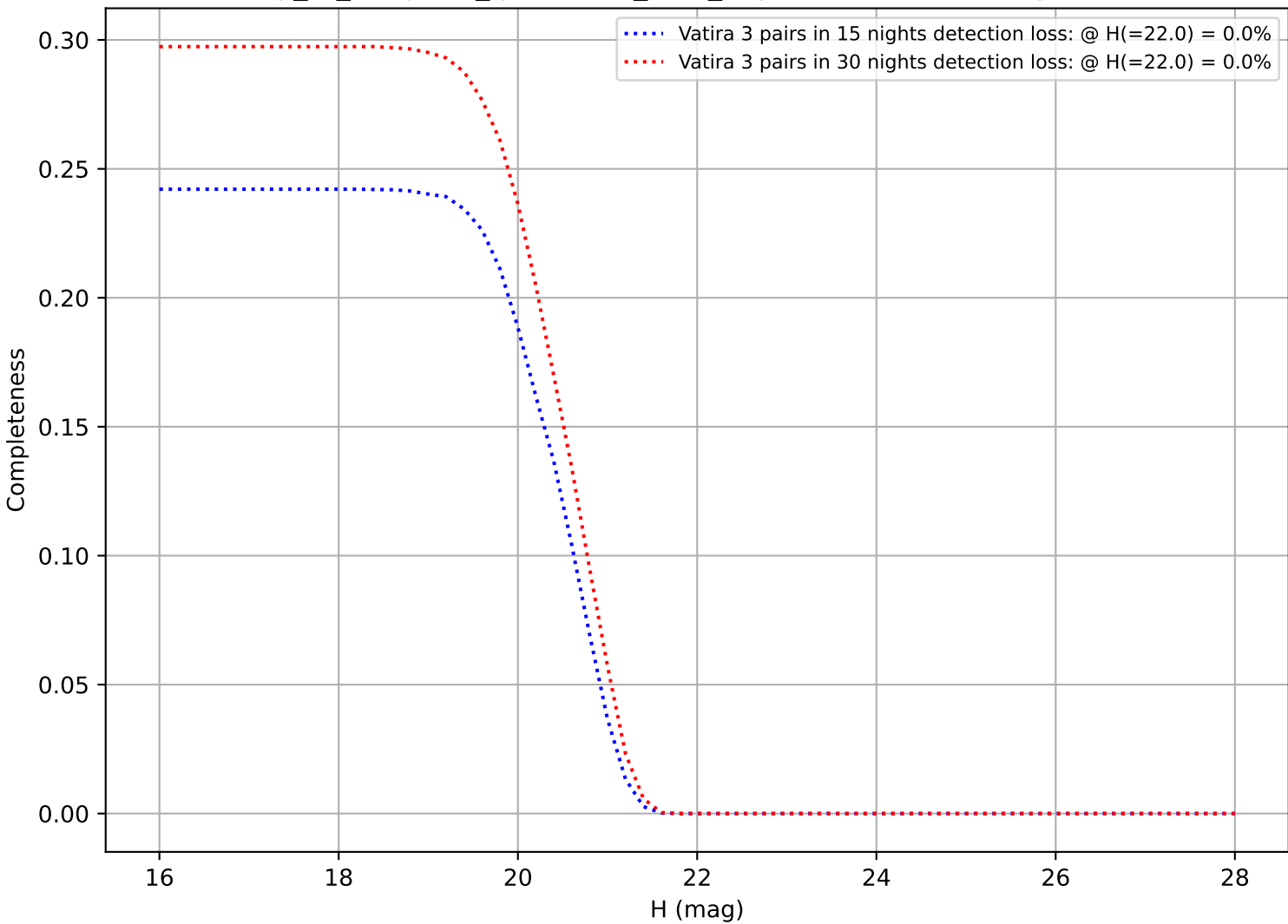
early_ss_template_fpextra3.0_v3.4_10yrs: DifferentialCompleteness
