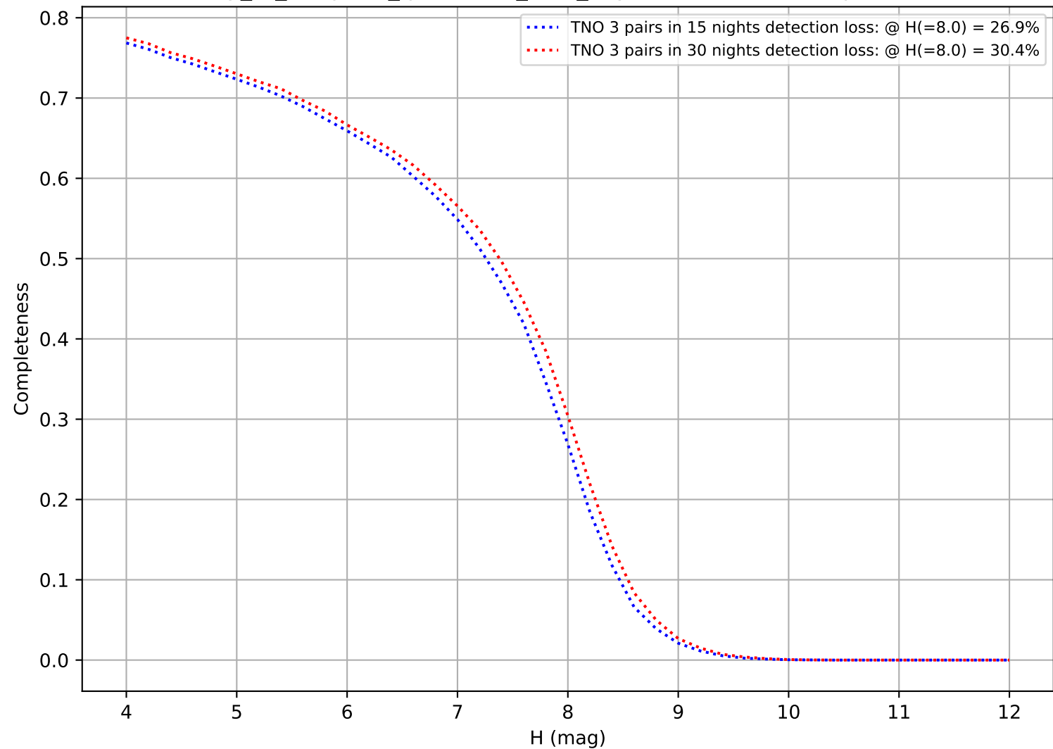
early_ss_template_fpextra3.0_v3.4_10yrs: DifferentialCompleteness
