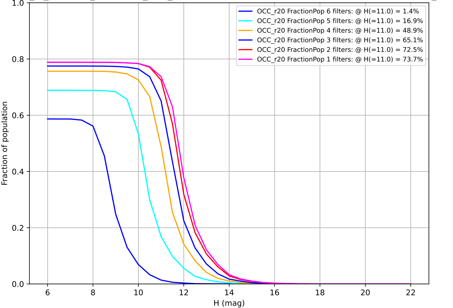
early_ss_template_fpextra3.0_v3.4_10yrs: Fraction of population with colors in X filters OCC_r20
