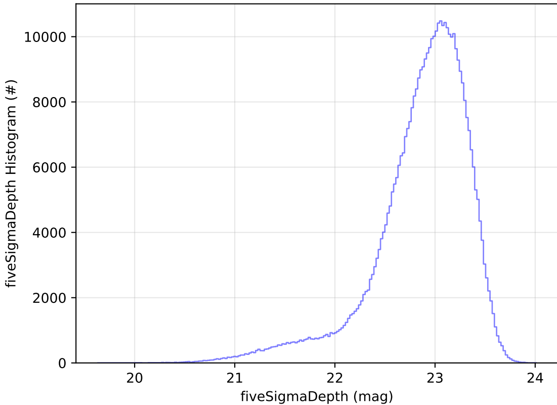
early_ss_template_fpextra3.0_v3.4_10yrs z: fiveSigmaDepth Histogram
