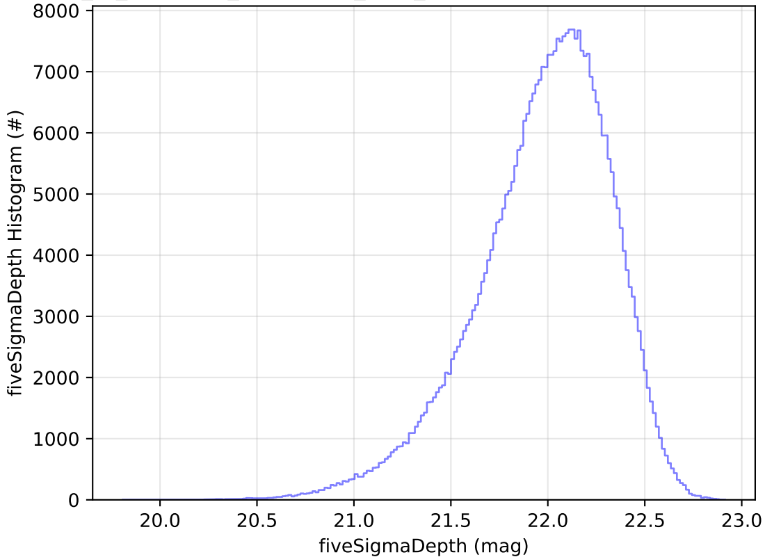
early_ss_template_fpextra3.0_v3.4_10yrs y: fiveSigmaDepth Histogram
