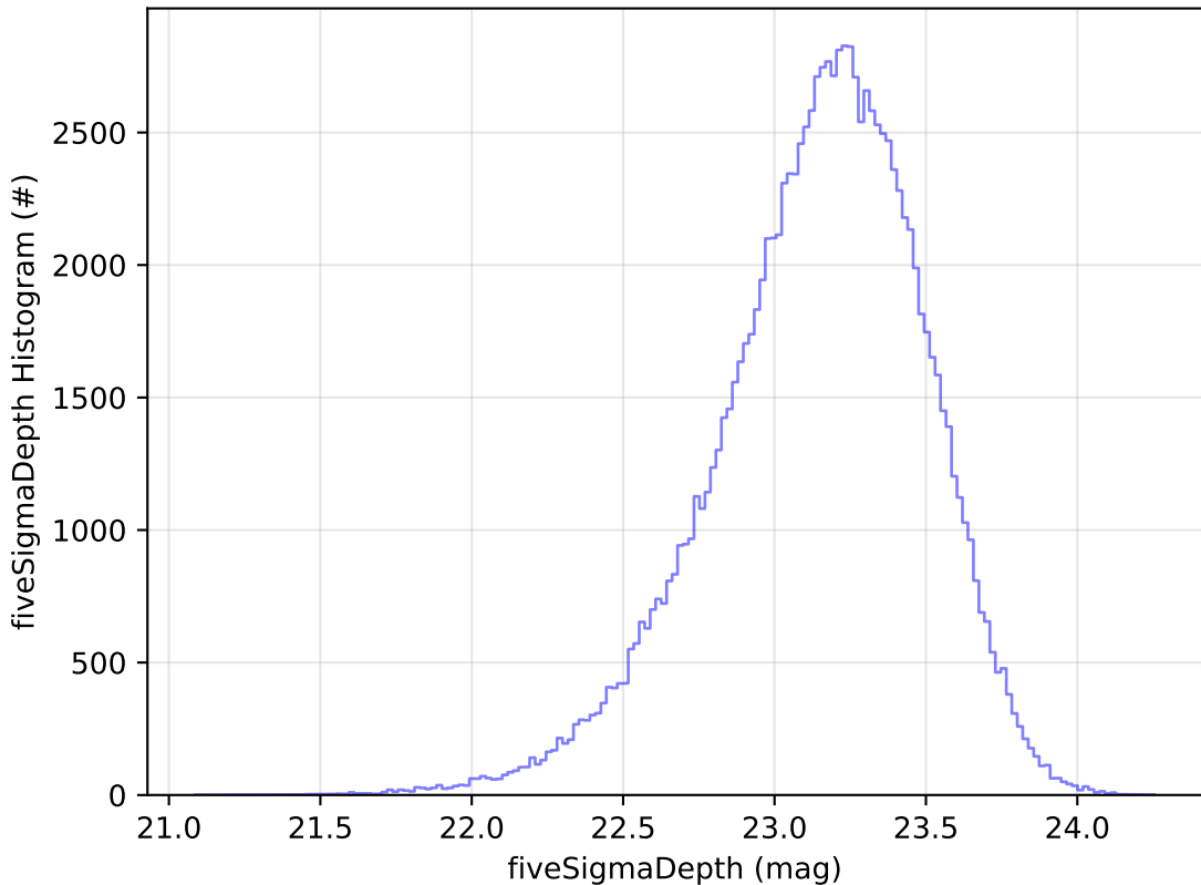
early_ss_template_fpextra3.0_v3.4_10yrs u: fiveSigmaDepth Histogram
