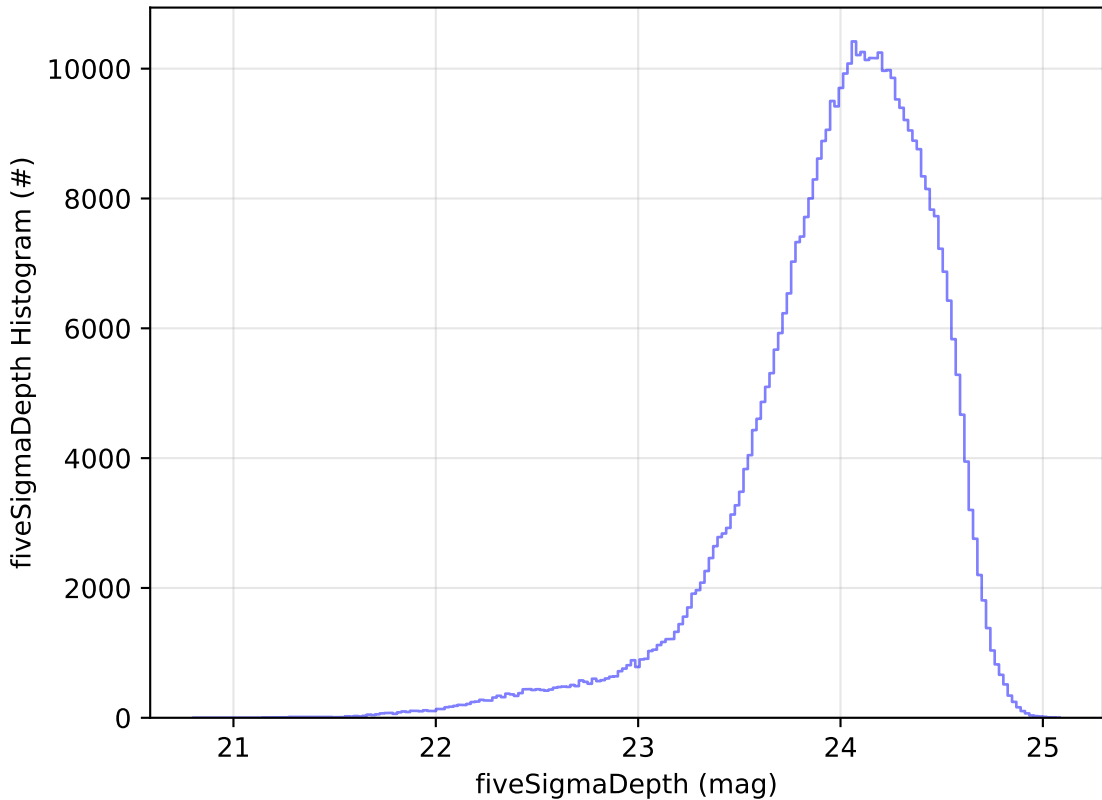
early_ss_template_fpextra3.0_v3.4_10yrs r: fiveSigmaDepth Histogram
