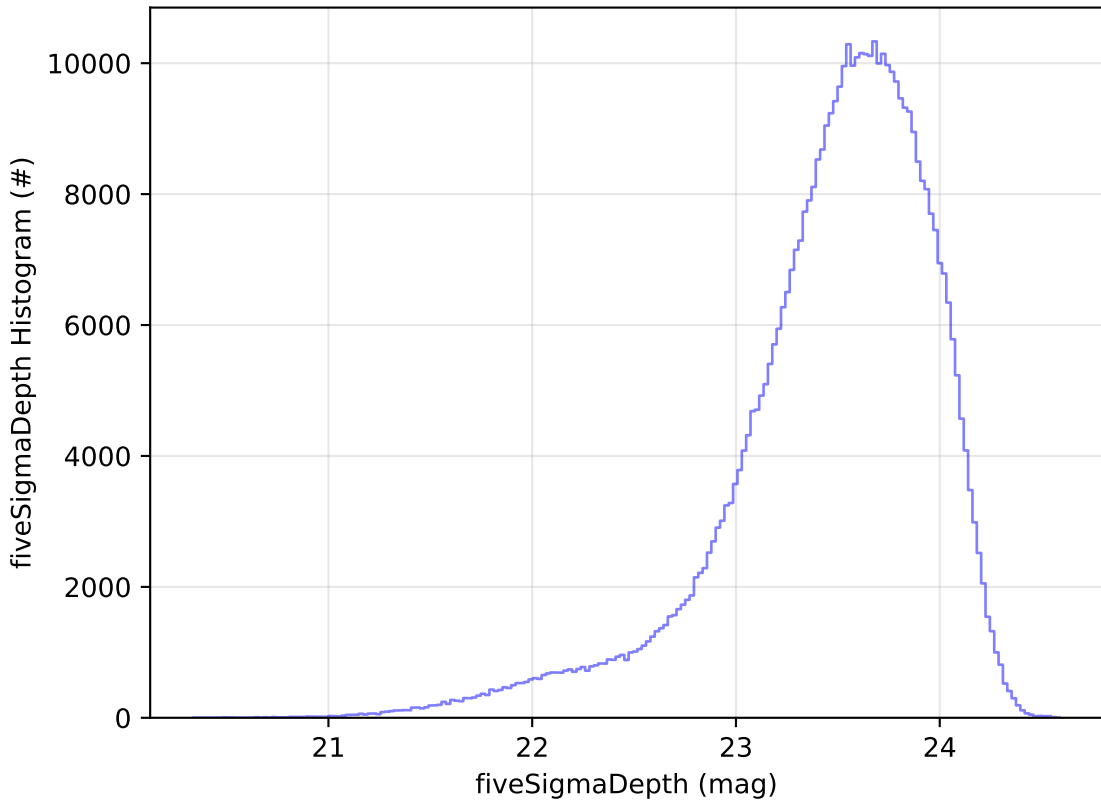
early_ss_template_fpextra3.0_v3.4_10yrs i: fiveSigmaDepth Histogram
