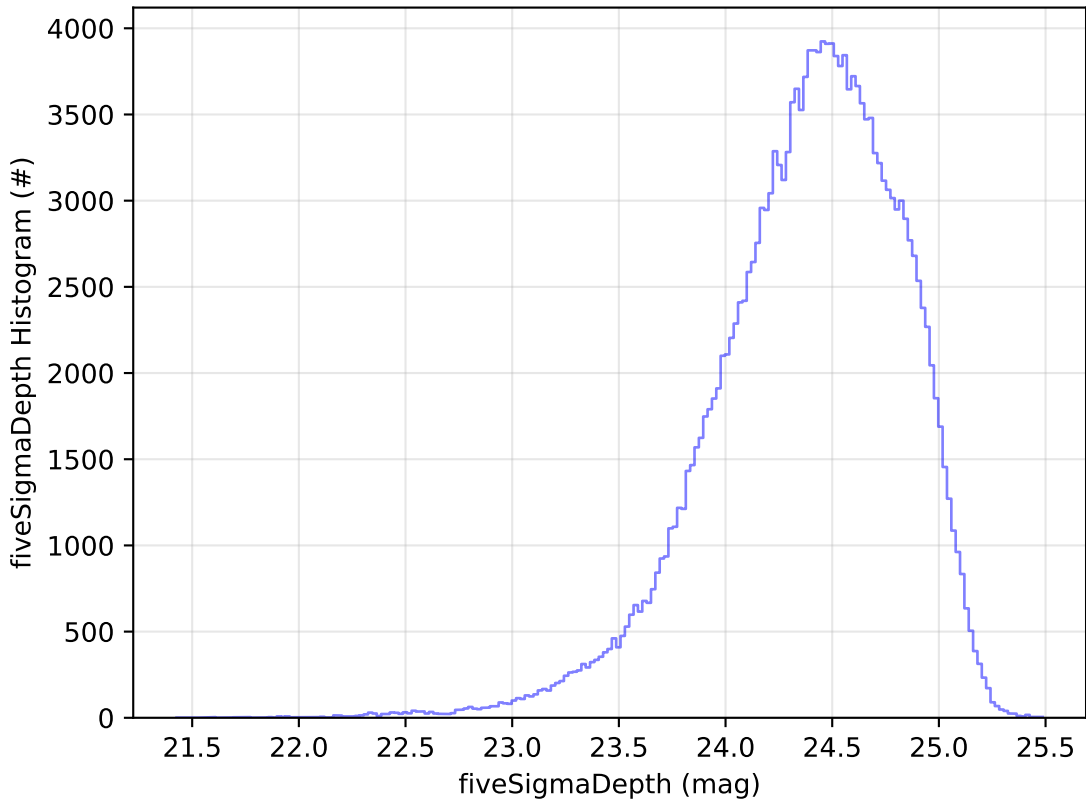
early_ss_template_fpextra3.0_v3.4_10yrs g: fiveSigmaDepth Histogram
