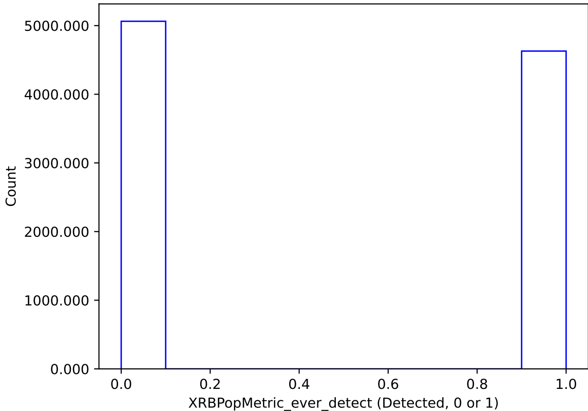
early_ss_template_fpextra3.0_v3.4_10yrs : XRBPoMetric_ever_detect
