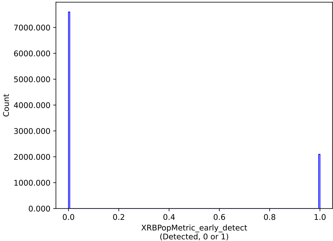
early_ss_template_fpextra3.0_v3.4_10yrs : XRBPoMetric_early_detect
