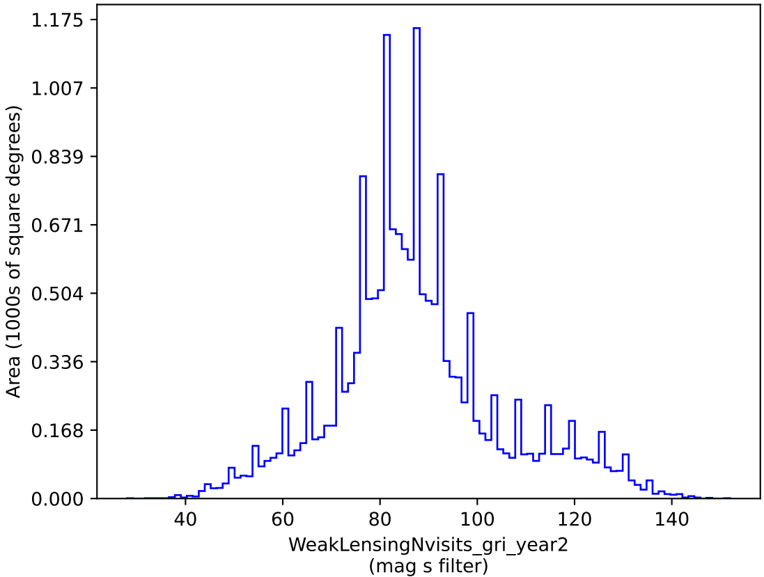
early_ss_template_fpextra3.0_v3.4_10yrs gri band non-DD: WeakLensingNvisits_gri_year2
