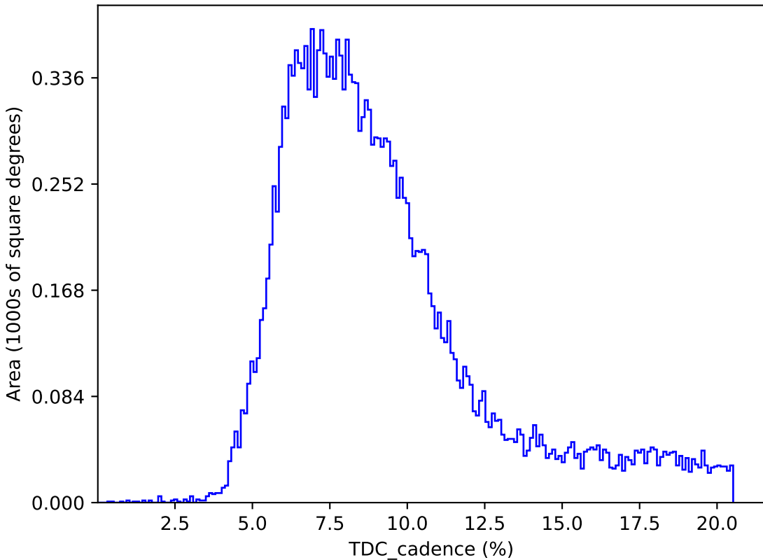
early_ss_template_fpextra3.0_v3.4_10yrs : TDC_cadence
