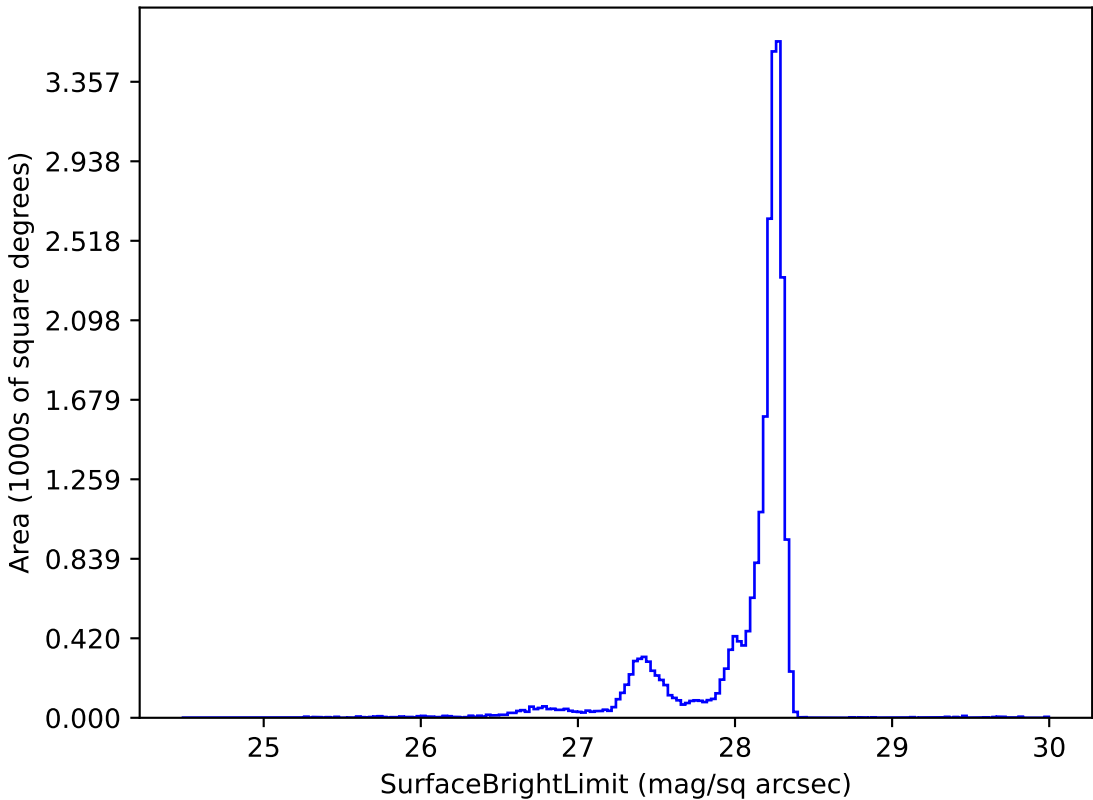
early_ss_template_fpextra3.0_v3.4_10yrs y: SurfaceBrightLimit
