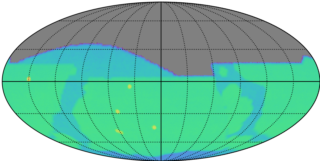
early_ss_template_fpextra3.0_v3.4_10yrs r: SurfaceBrightLimit
