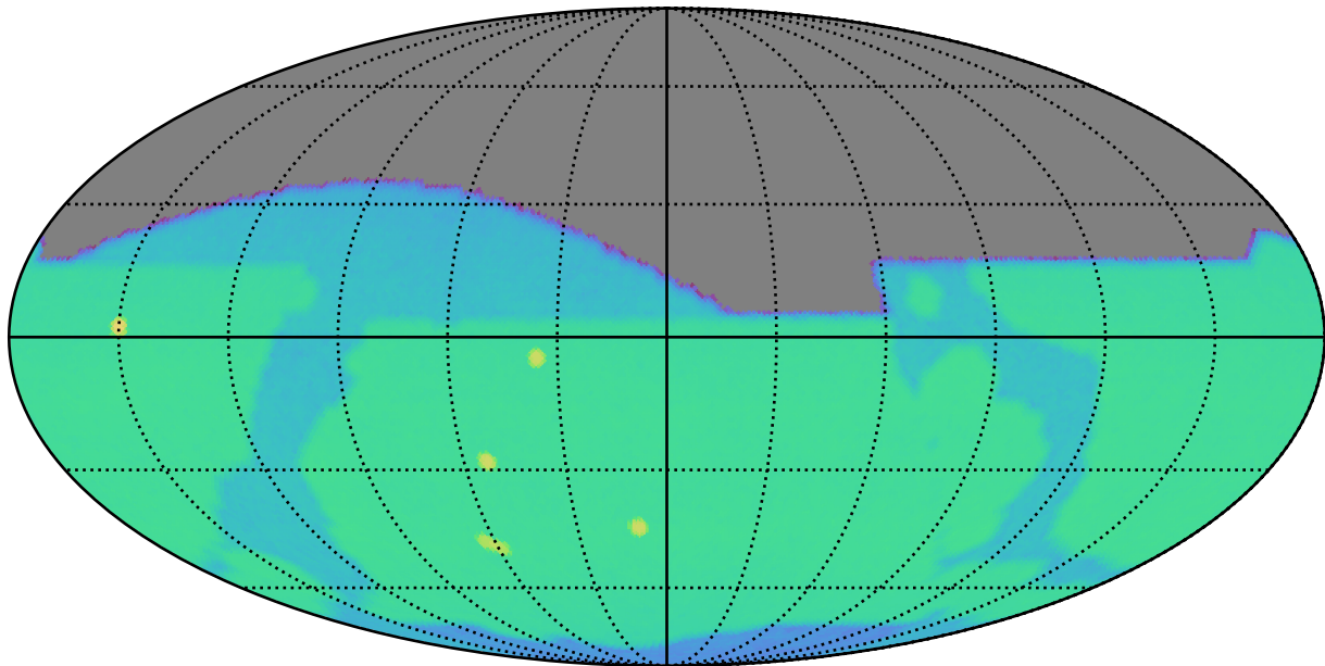
early_ss_template_fpextra3.0_v3.4_10yrs i: SurfaceBrightLimit
