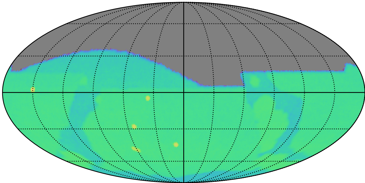
early_ss_template_fpextra3.0_v3.4_10yrs g: SurfaceBrightLimit
