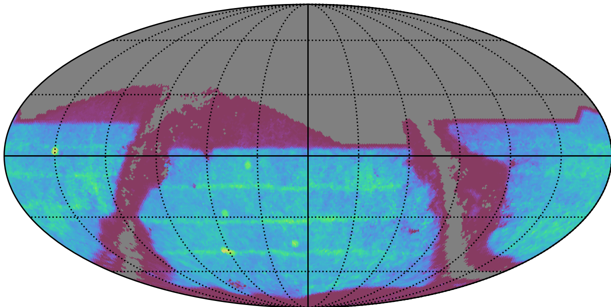
early_ss_template_fpextra3.0_v3.4_10yrs : SNSLMetric
