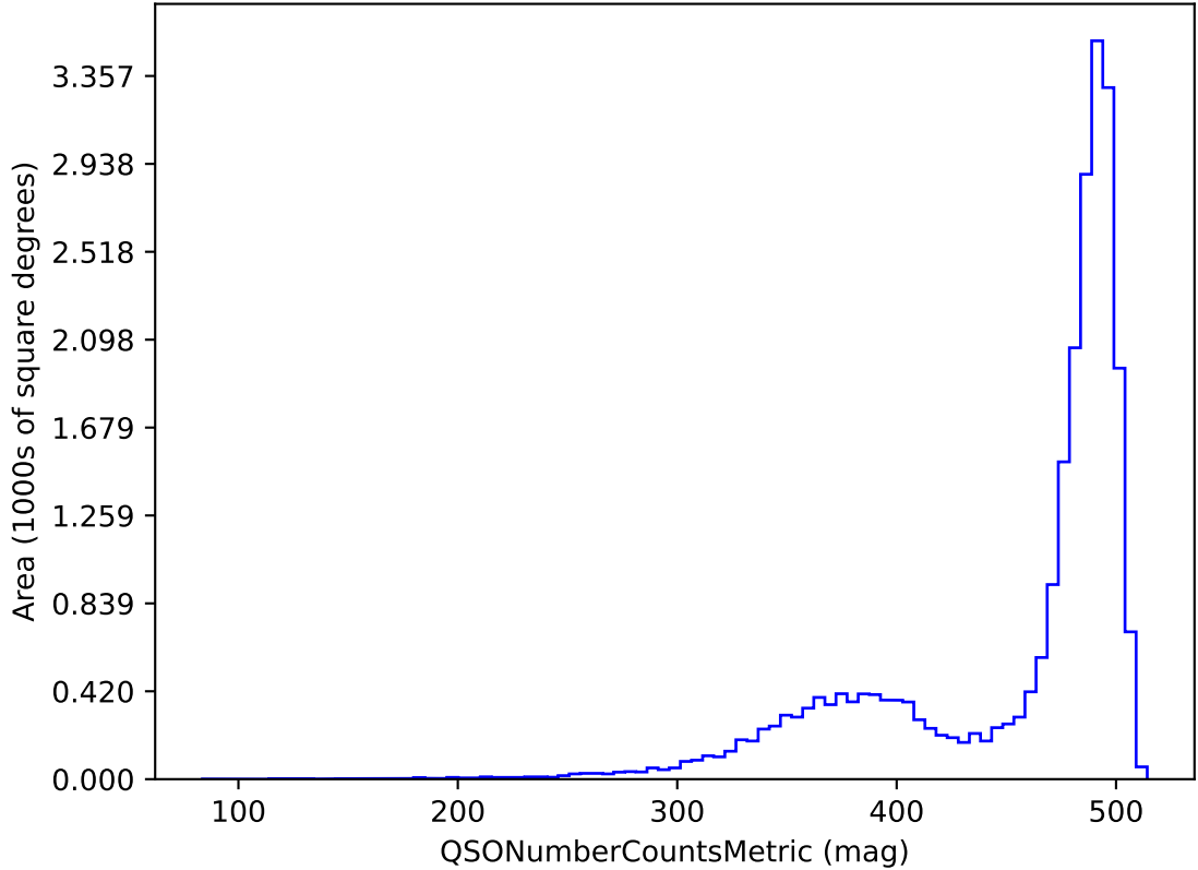
early_ss_template_fpextra3.0_v3.4_10yrs z band and non-DD: QSONumberCountsMetric
