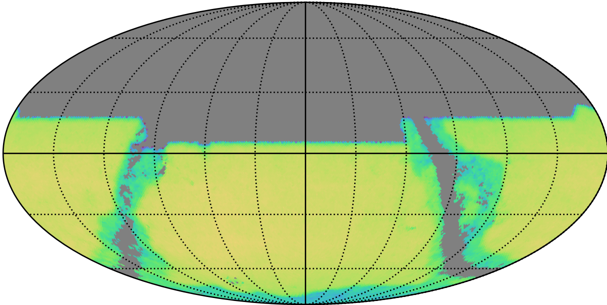
early_ss_template_fpextra3.0_v3.4_10yrs y band and non-DD: QSONumberCountsMetric
