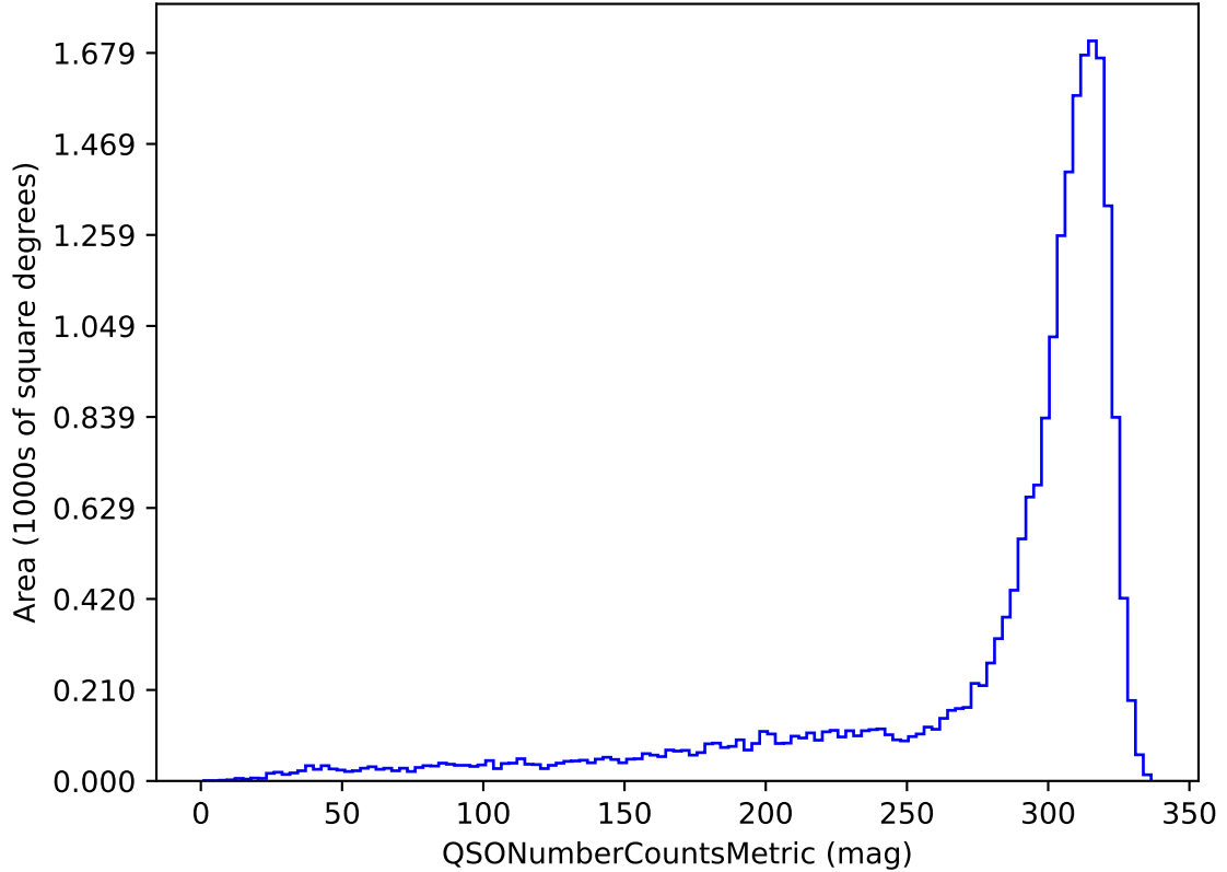
early_ss_template_fpextra3.0_v3.4_10yrs u band and non-DD: QSONumberCountsMetric
