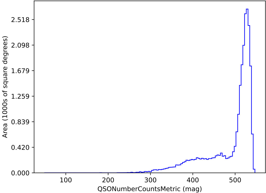
early_ss_template_fpextra3.0_v3.4_10yrs r band and non-DD: QSONumberCountsMetric
