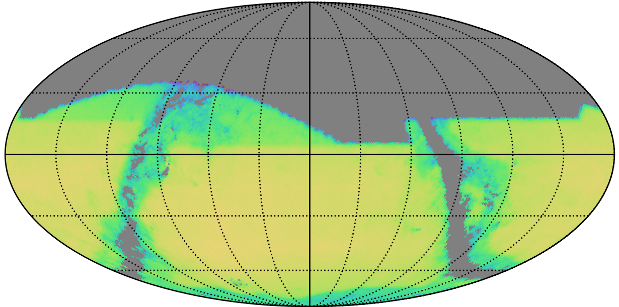
early_ss_template_fpextra3.0_v3.4_10yrs i band and non-DD: QSONumberCountsMetric
