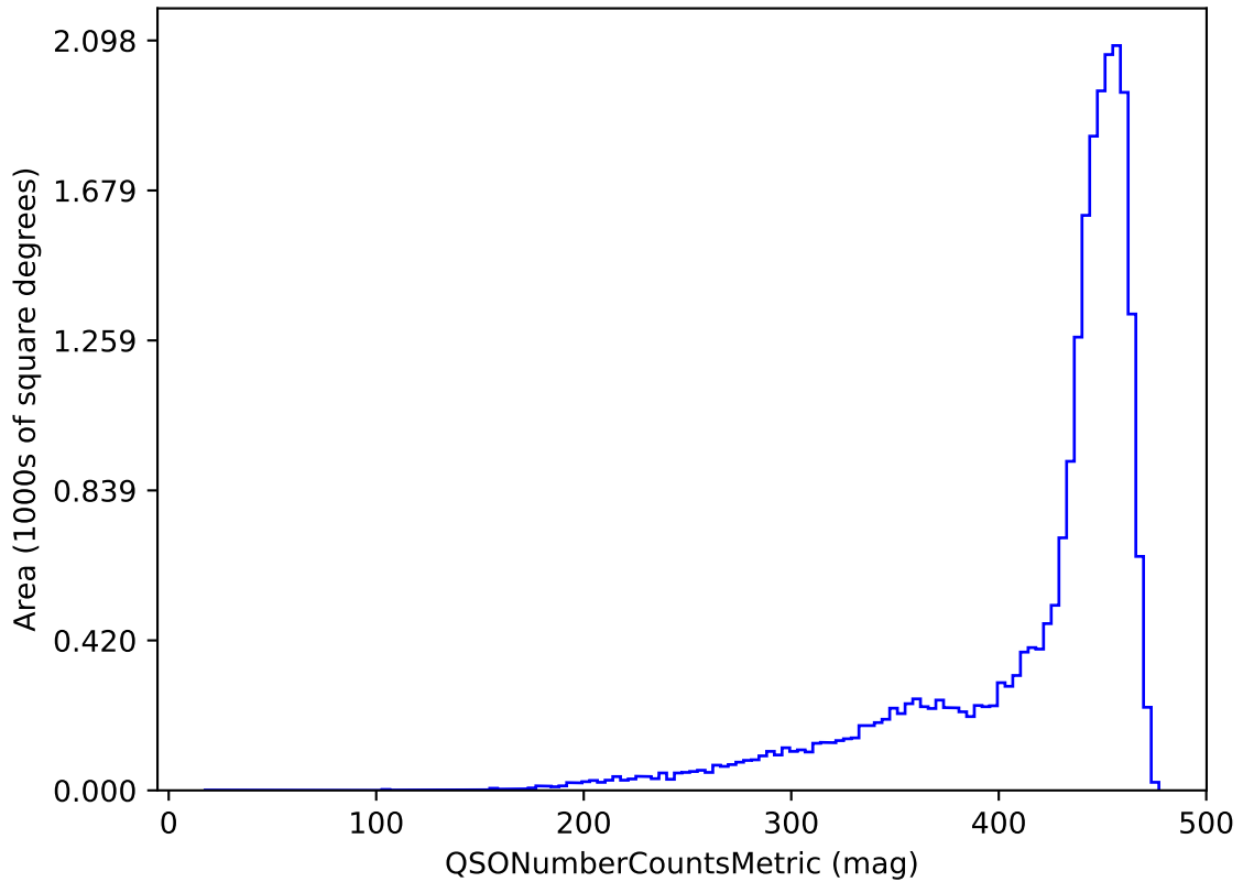
early_ss_template_fpextra3.0_v3.4_10yrs g band and non-DD: QSONumberCountsMetric
