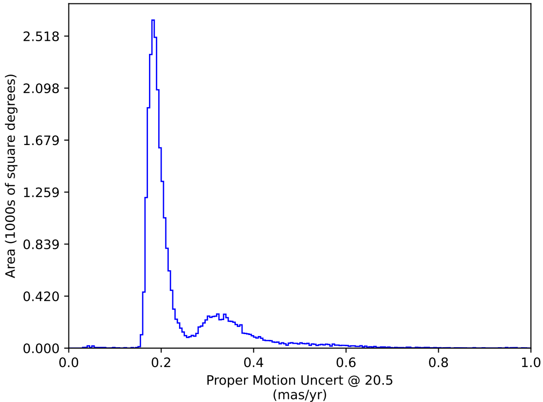
early_ss_template_fpextra3.0_v3.4_10yrs : Proper Motion Uncert @ 20.5
