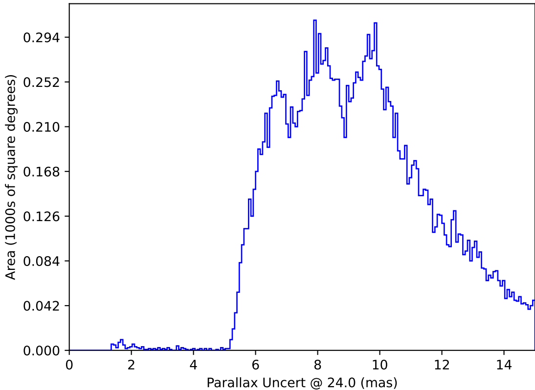
early_ss_template_fpextra3.0_v3.4_10yrs : Parallax Uncert @ 24.0
