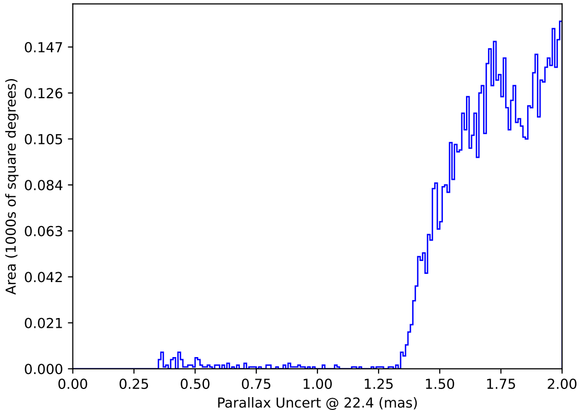
early_ss_template_fpextra3.0_v3.4_10yrs : Parallax Uncert @ 22.4
