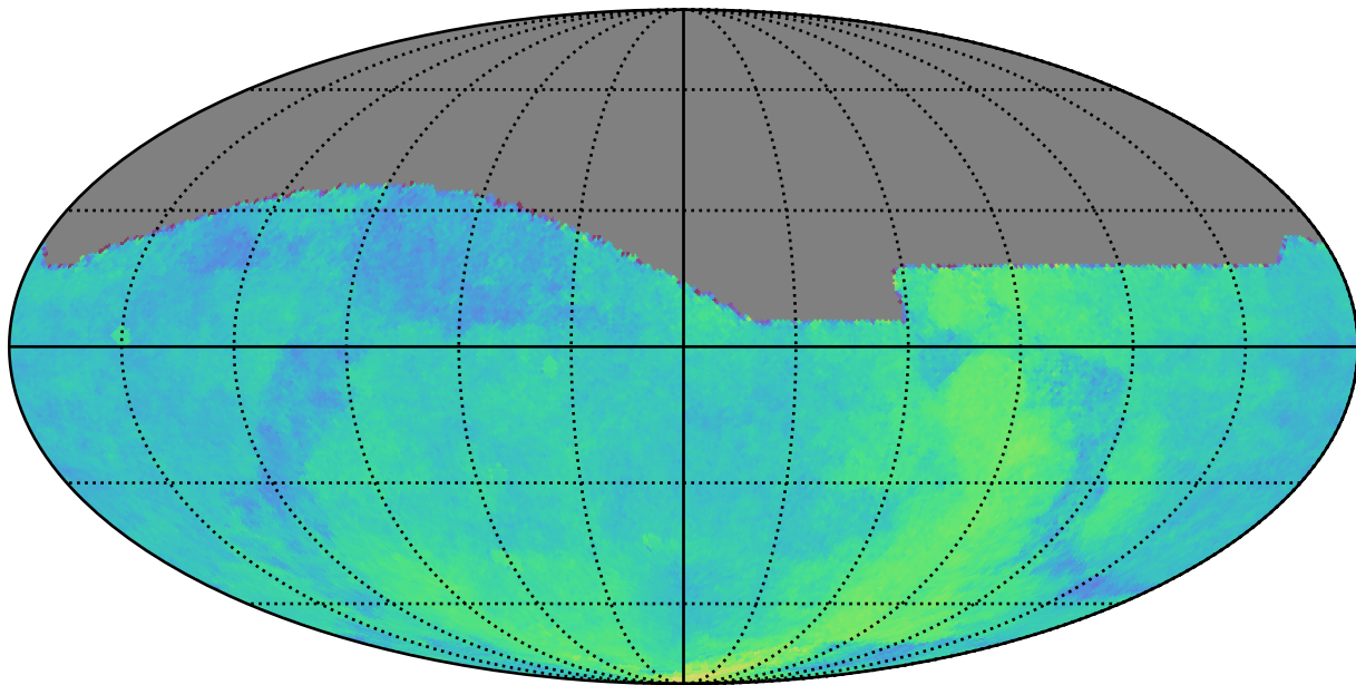
early_ss_template_fpextra3.0_v3.4_10yrs : Parallax Coverage @ 24.0
