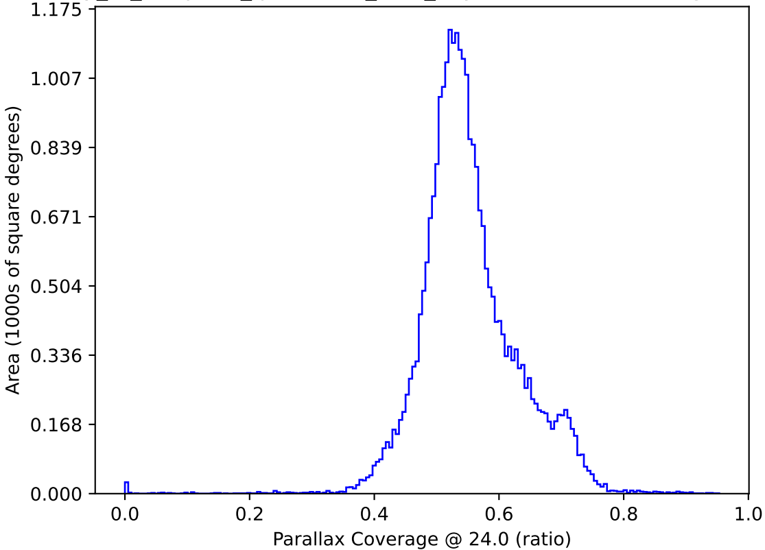
early_ss_template_fpextra3.0_v3.4_10yrs : Parallax Coverage @ 24.0
