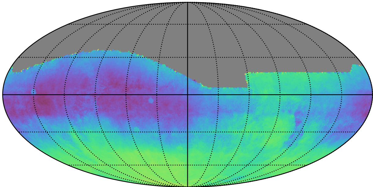
early_ss_template_fpextra3.0_v3.4_10yrs : Parallax-DCR degeneracy @ 24.0
